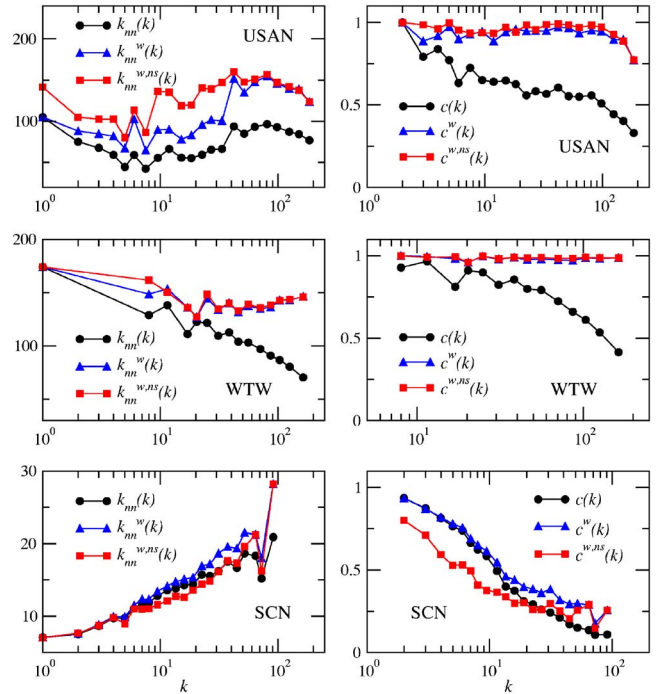
FIG. 2. (Color online) Correlation measures for real networks. From top to bottom, the U.S. airport network (USAN) for the year 2005, the world trade web (WTW) for the year 2000, and the scientific collaboration network (SCN).
