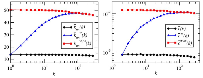
FIG. 1. (Color online) Correlation measures for a random WCN generated with the algorithm defined in the text with P(k) \sim k^{-2.5} and \bar{s}(k) \propto k^{1.5} .
